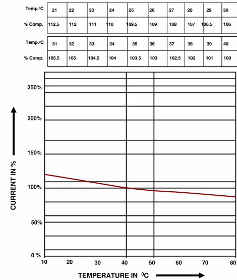
Ambient Compensation Curve (TAB-2)
