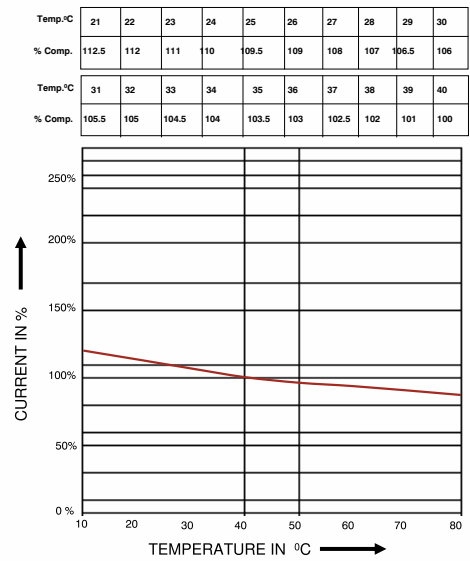
Ambient Compensation Curve (TAB-1)
